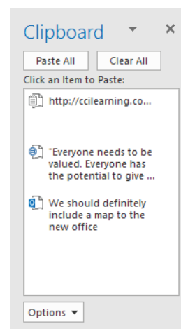
Window/Task Pane
