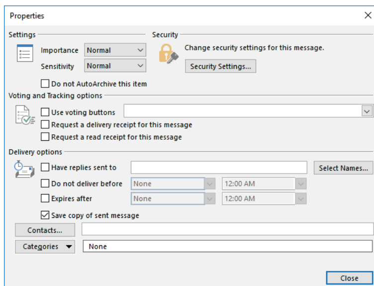
Dialog Box
